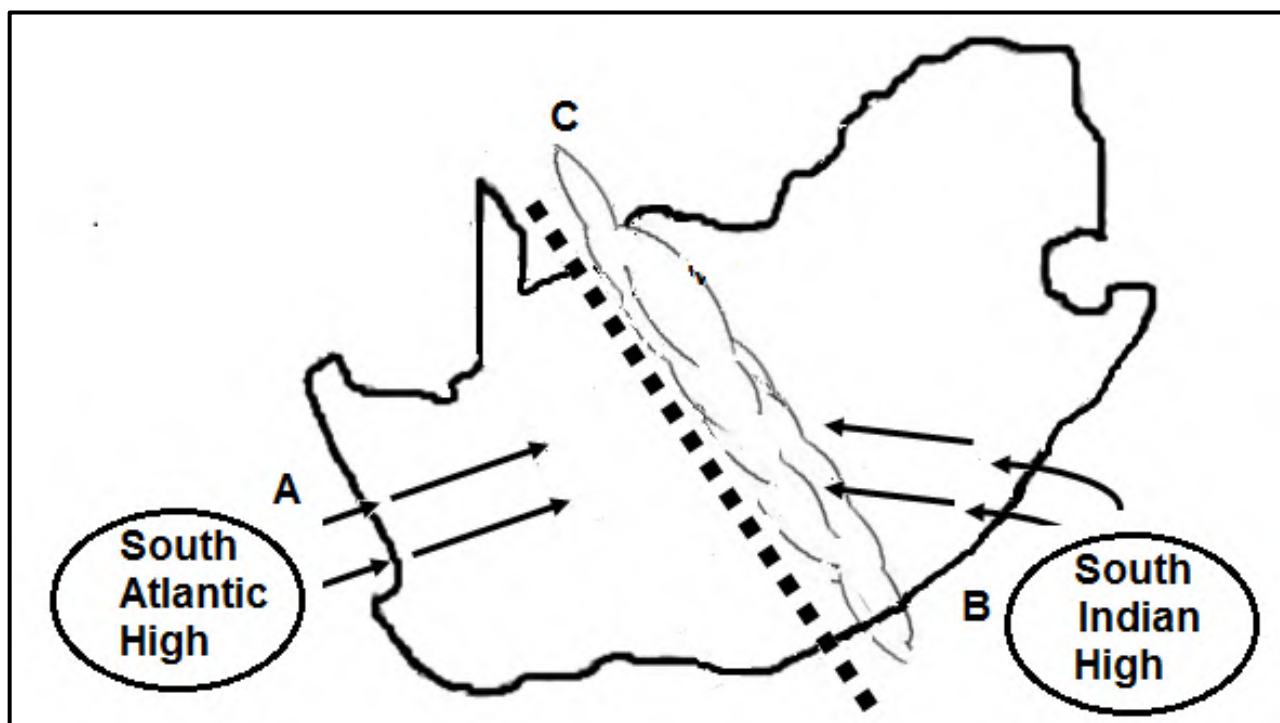
FIGURE 1.4: LINE THUNDERSTORM
