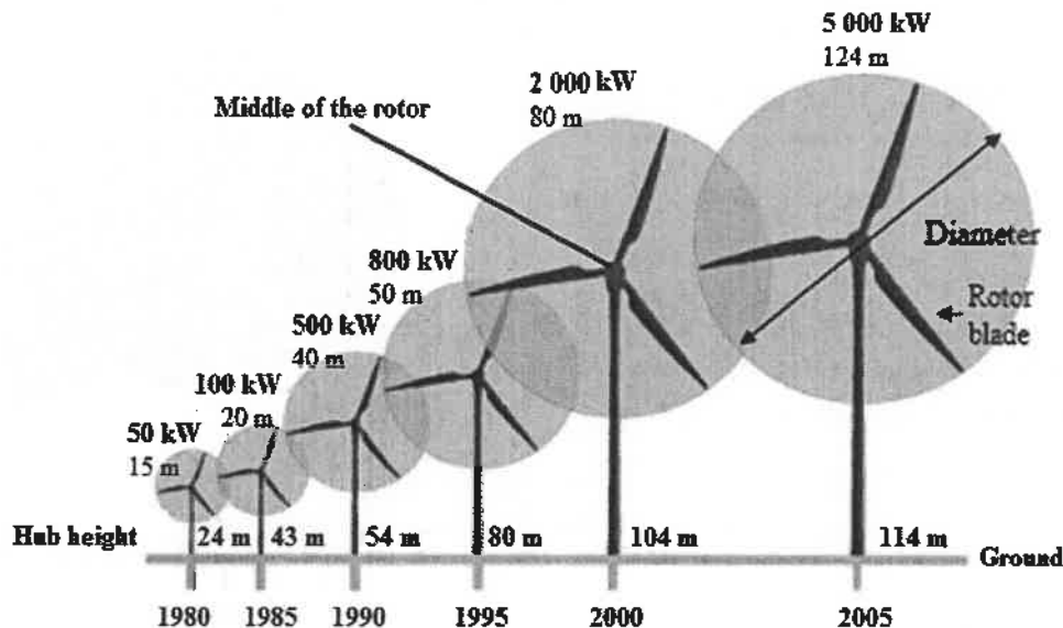
PICTURES OF WIND TURBINES AND GENERATION CAPACITY USED FROM 1980 to 2005
