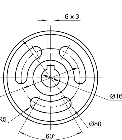
ADJUSTING HAND WHEEL [4]
