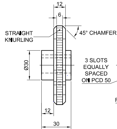
ADJUSTING HAND WHEEL [4]
