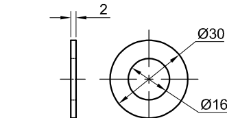
WASHER [6]
