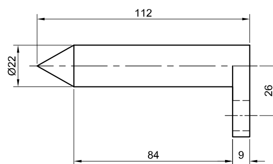
DEAD CENTRE [2]
