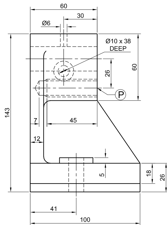
TAILSTOCK [1]
